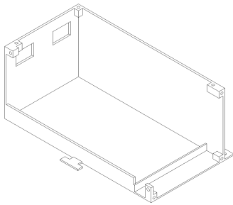
Base Body - Right
