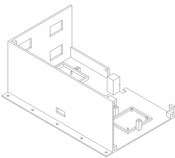
Base Body - Left
